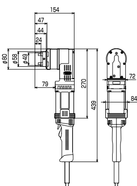
GMC-221EZ GMC-222EZ
